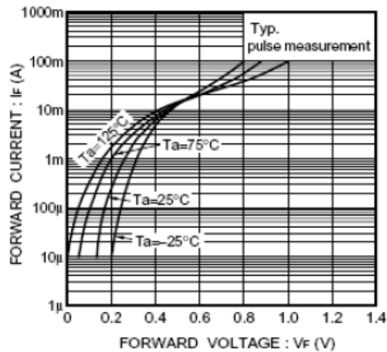
Fig. 1 Forward characteristics
